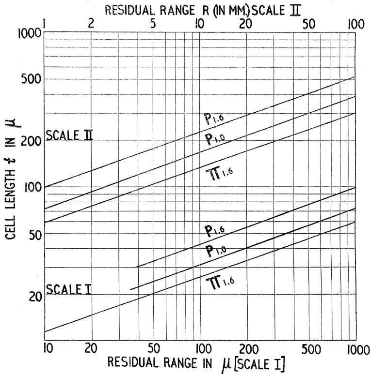
FIG. 1. The variation of the cell-length, t with Residual Range R for constant value of the mean absolute second difference, \Delta . The curves correspond to \Delta=1.6 \mu for protons and \pi -mesons and to \Delta=1.0 \mu for protons.
